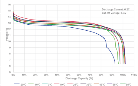
Discharge Capacity at Different Temperatures
